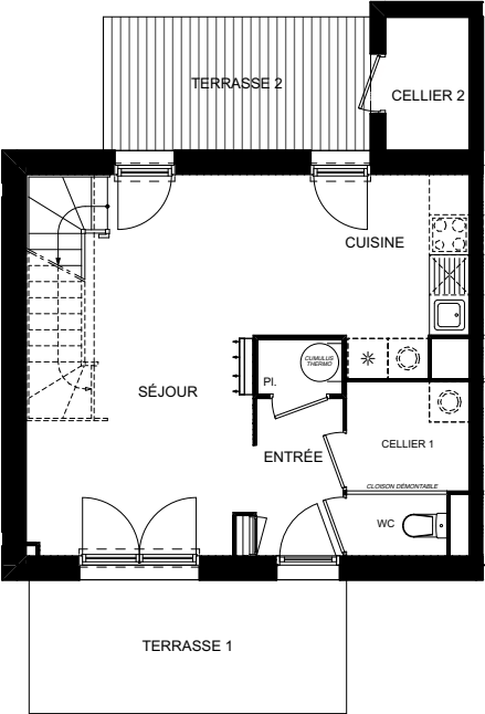
RDC - BASE
